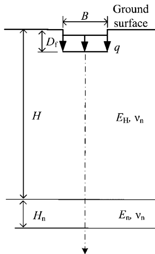
Figure 4. Equivalent two-layered soil systems for Figure 3.
