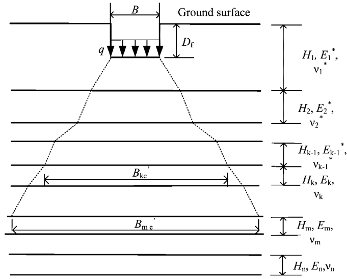
Figure 15. Distribution widths of vertical stress for Figure 13.
